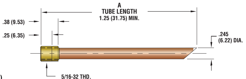
FIGURE 7-8 (Material - Copper & Brass)
