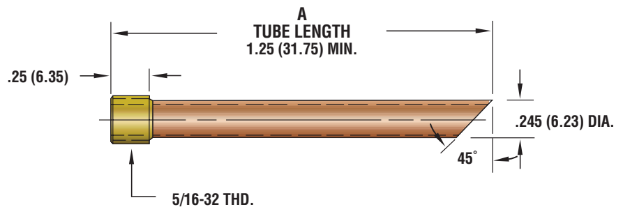
FIGURE 7-4 (Material - Copper & Brass)
