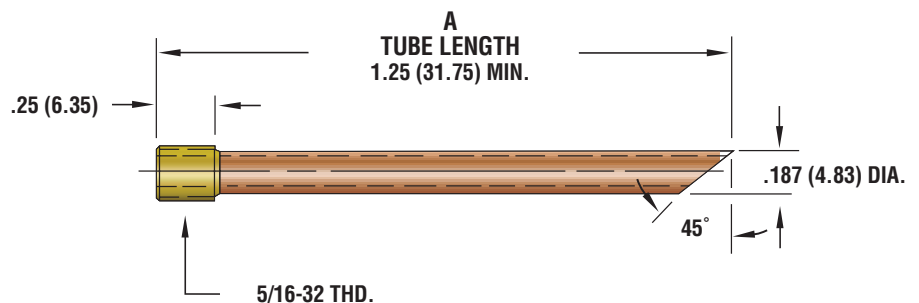
FIGURE 7-5 (Material - Copper & Brass)
